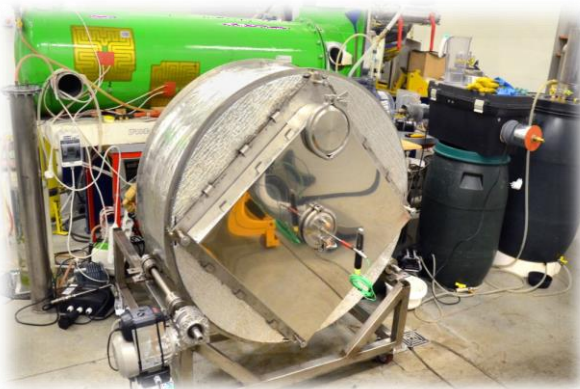
Pilot-scale anaerobic bioreactor (fermenter)
